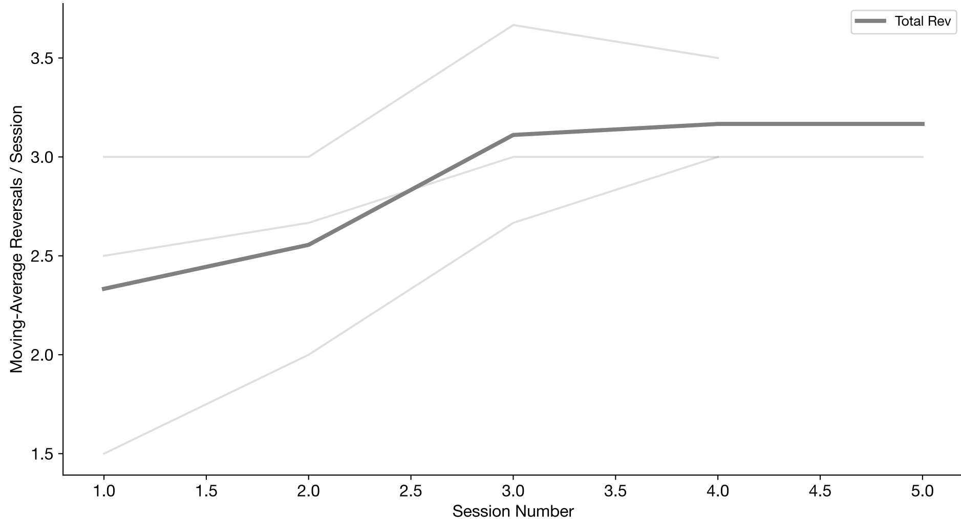
Moving-Average Total Reversals Over Time (n=3 subjects; sessions per subject=4–5; window=3)
